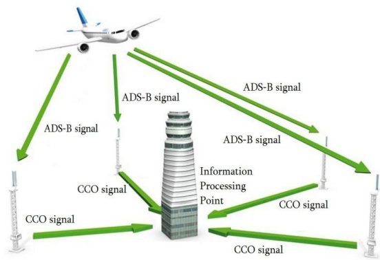
Figure 1: ADS-B receiver system layout using MLAT technologies
