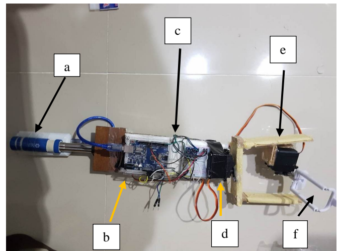
Figure 3: The Final result of the smartphone holder tool with gimbal system (a) The stick and the power bank as the power provider for the Arduino, (b) Arduino Uno location, (c) MPU6050 Gyro Sensor Location, (d) Roll axis servo location, (e) Servo drive location the pitch axis, (f) The bracket where the smartphone is placed
