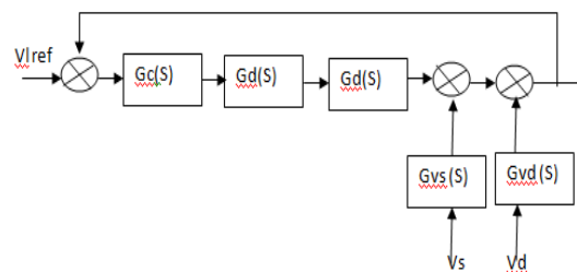
Fig 5 Block diagram of the load voltage control using DSTATCOM or DVR
