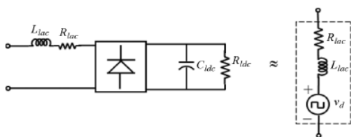
Fig 3: Voltage source type of the nonlinear load.
