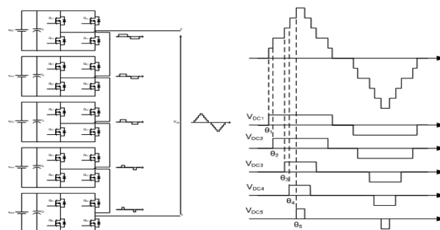
Fig. 13. Single -phase eleven -level cascaded transformer H-bridge VSC.
