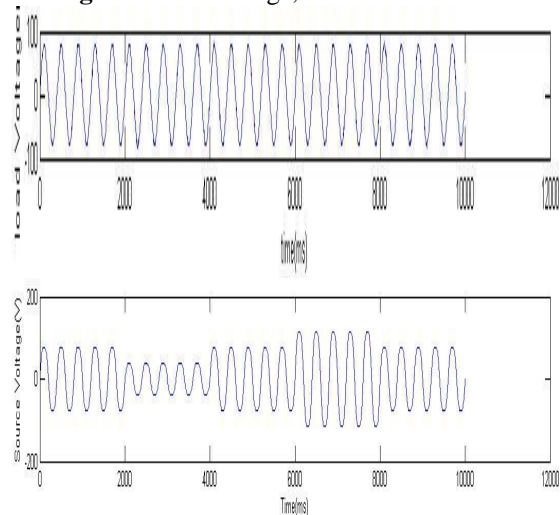
Fig 12: Load voltage Source voltage
