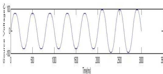
Fig 9: Source voltage
