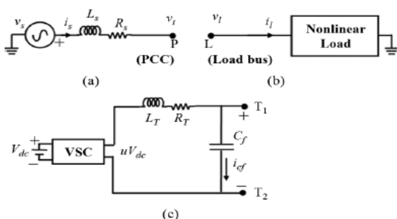
Fig 4: Compensator structure used for load voltage control for a single-phase equivalent of a distribution system. (a) Feeder. (b) Load. (c) Compensator.
