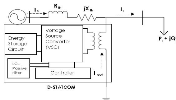
Fig 2 : System scheme for d-statcom
