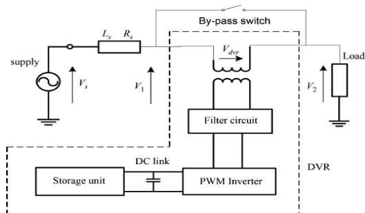
Fig 1: Schematic Circuit of Dynamic Voltage Restorer
