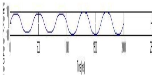
Fig 9: Source voltage
