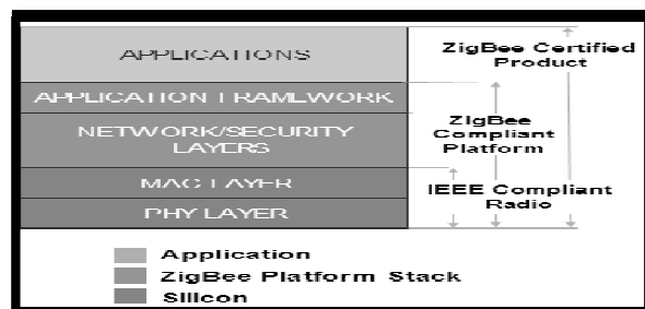
Fig 5. ZigBee Stack Protocol
