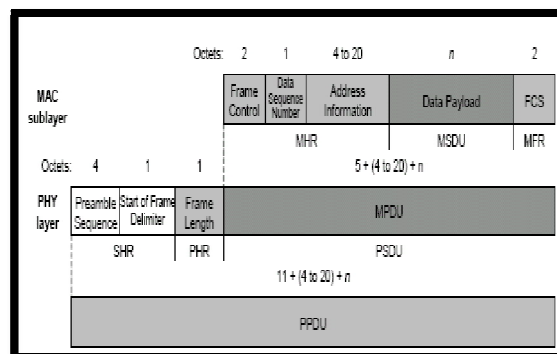
Fig.6 ZigBee Layers
