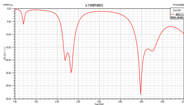
Fig.4 Return loss ( S_{11} ) parameter of the unequal E-shape antenna
