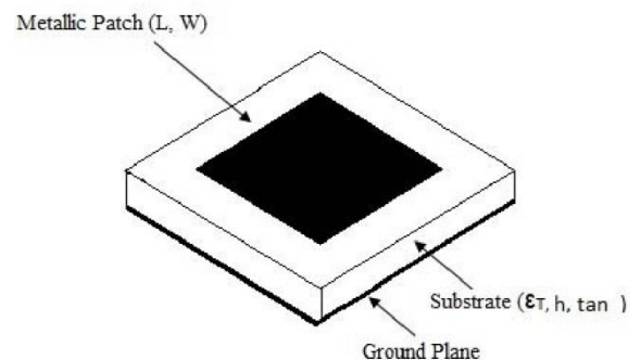
Figure 1.1 Microstrip Antenna
