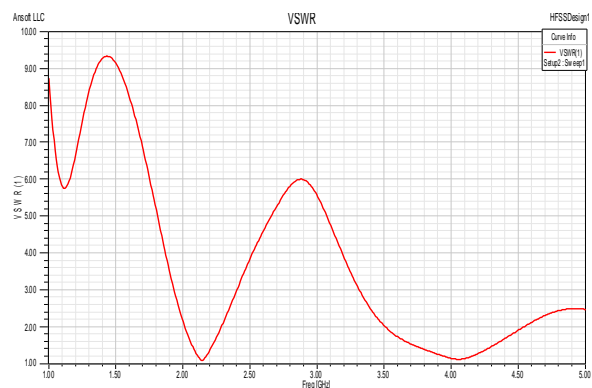
Fig.6 VSWR of the unequal E-shape antenna
