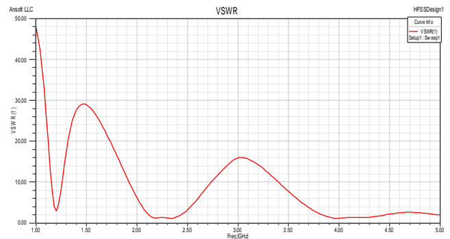
Fig.6 VSWR of the unequal E-shape antenna
