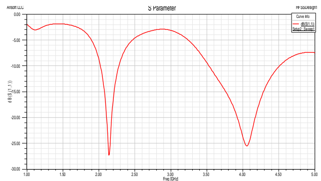
Fig.5 Return loss( S_{11} ) parameter of the stacked antenna
