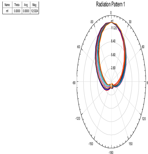
Fig.8. Radiation pattern of the stacked antenna
