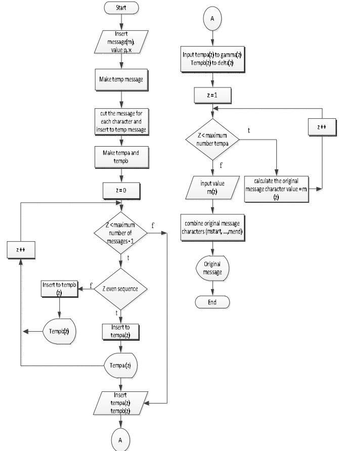
Figure 6: Decryption Process Flowchart
