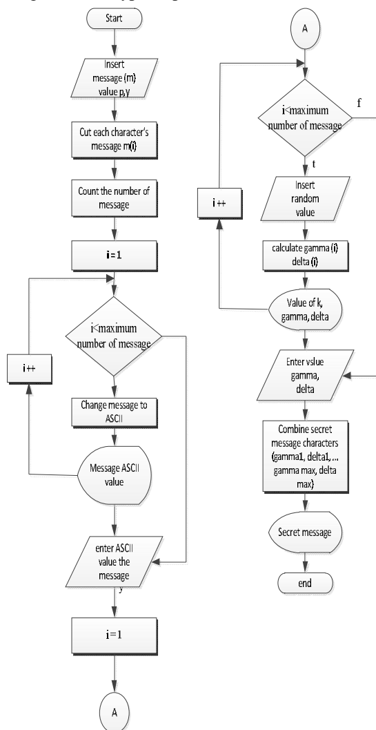
Figure 5: Encryption Process Flowchart
