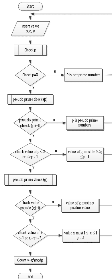
Figure 4: Key Formation Flowchart
