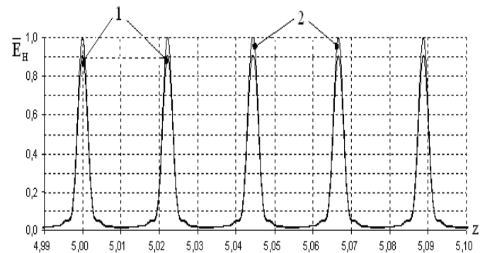
Figure 3. Impact of errors \Delta\rho and \Delta h on the distribution of the electric field strength of a cylindrical phased antenna array along the range at \nu = 4 ( Q = 12 )
