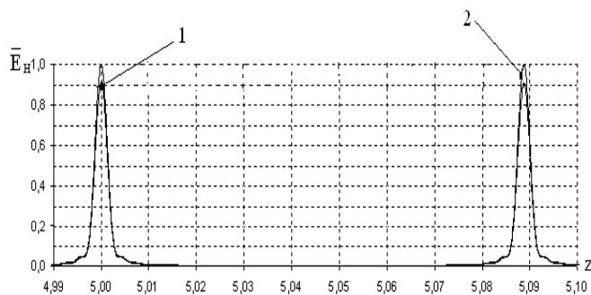
Figure 2. Impact of errors \Delta\rho and \Delta h on the distribution of the electric field of the phased array antenna by range (1 – \Delta\rho=0; \Delta h =\lambda/6 )
