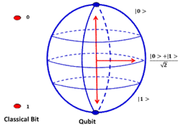
Figure 1: Comparing Classical bit and Qubit Source: [14]
