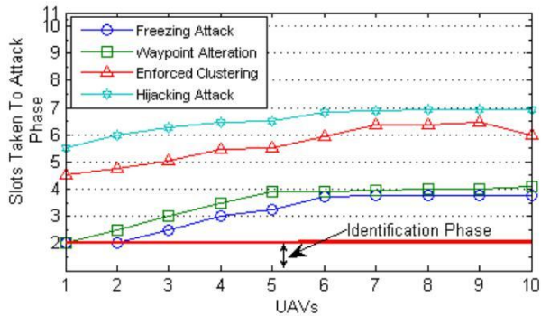
Figure 3: Slot requirement for coagulation attack with fixed topology.
