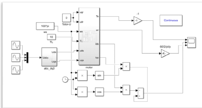
Figure 1: Simulation model of asynchronous motor rotor bar breaking
