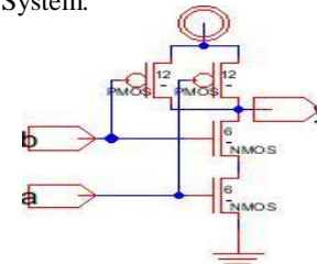
Fig 4:Schematic Diagram of a 2-inputNand gate
