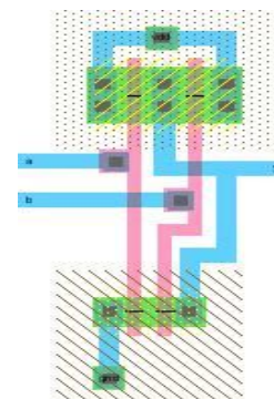
Fig 5:Layout design of a 2-input NAND gate
