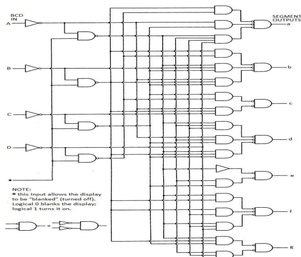
Fig:2 The logic diagram of 7 segment decoder
