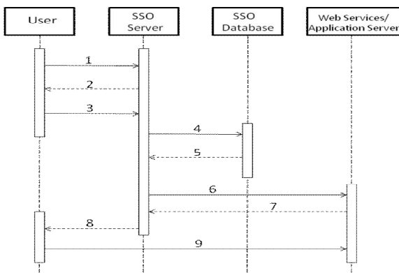
Figure 2: Sequence Diagram of SSO System
