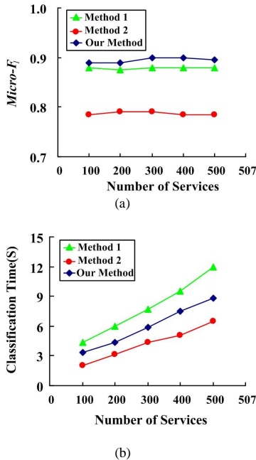
Fig. 3. Comparison with other classification methods
