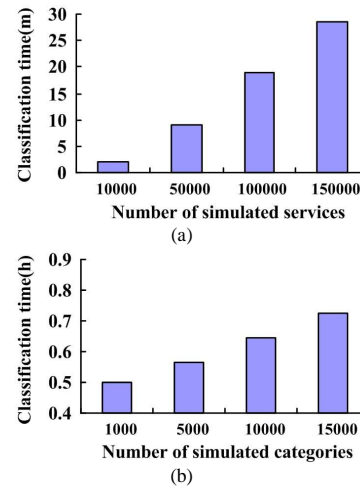
Fig. 4. Scalability of our classification method
