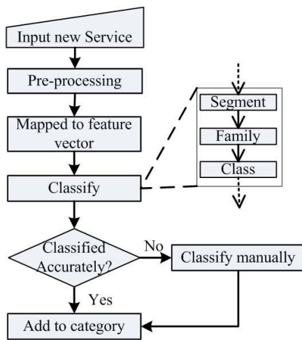
Fig. 1. The complete process of service classification
