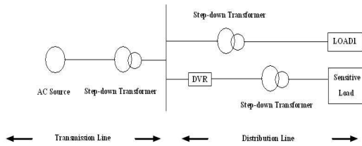
Fig. 1 Location of DVR
