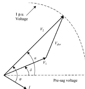
Fig. 3 Phasor diagram of electrical conditions during a voltage sag
