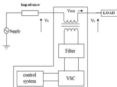
Fig. 2 Schematic diagram of DVR
