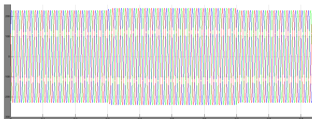
Fig. 6 Voltage swell without DVR
