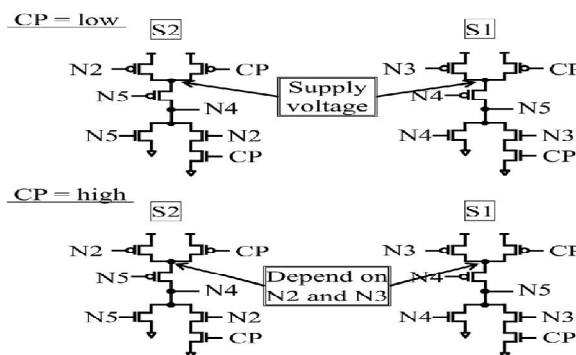
Fig. 12. The state of internal nodes.
