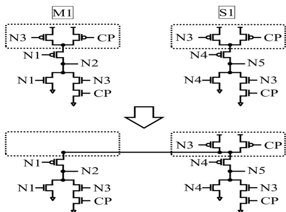
Fig. 9. Transistor merging in PMOS side.
