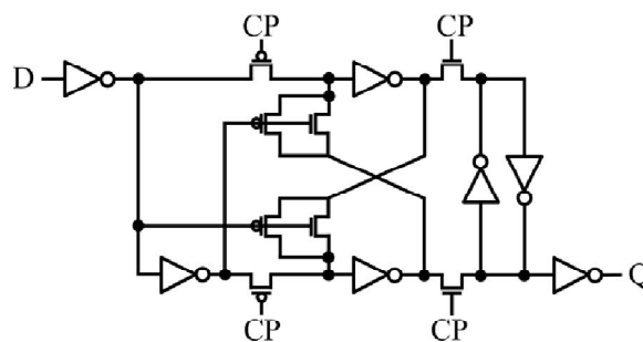
Fig. 5. Adaptive-coupling flip-flop (ACFF).
