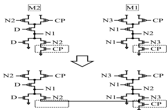
Fig. 10. Transistor merging in NMOS side.
