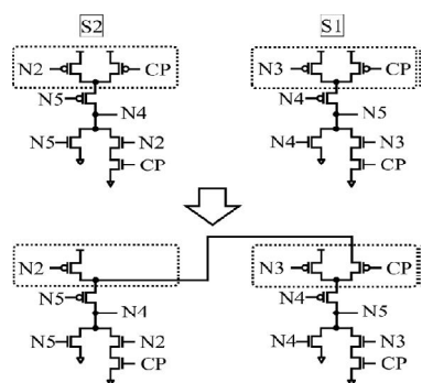
Fig. 11. Further transistor merging in PMOS side.
