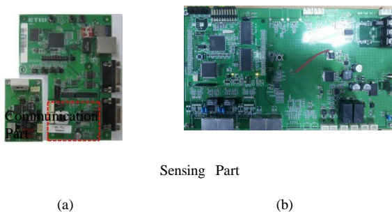
Figure 10. Components for renewable energy monitoring. (a) PLC modem, (b) Renewable energy gateway (REG).
