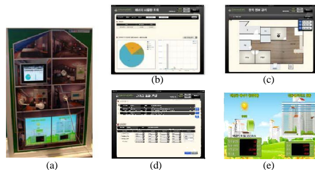
Figure. 7. Home server user interfaces. (a) Test set, (b) Energy usages of home appliances and lights, (c) Mapping information, (d) Device lists, (e) Solar power system information.
