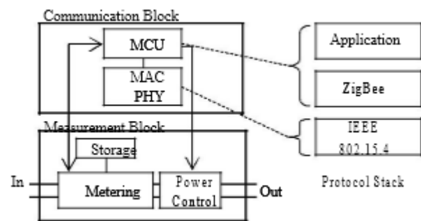
Figure. 3. Energy measurement and communication unit (EMCU) and protocol stack.
