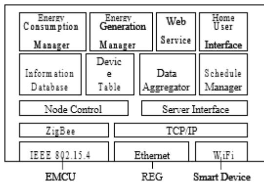
Figure. 2. Function blocks of a home server.
