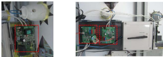
Figure 9. Energy management and communication unit (EMCU) installed in the miniaturized test set.
