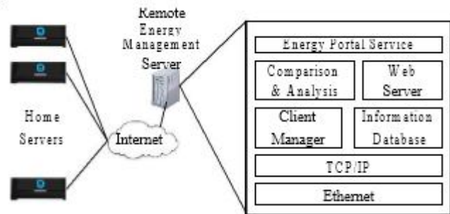
Figure. 6. Remote energy management server (REMS) connected to the home servers of subscribing clients.
