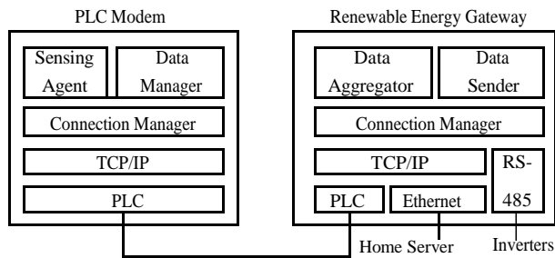
Figure. 5. Architecture of a renewable energy gateway (REG) and a PLC modem.
