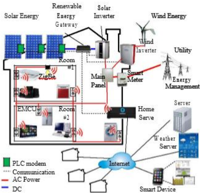
Figure. 1. Architecture of smart home energy management (HEMS) considering both energy consumption and generation.
